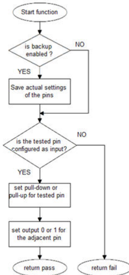
Figure 14. Block diagram of FS_DIO_ShortToAdjSet_LPC() function
