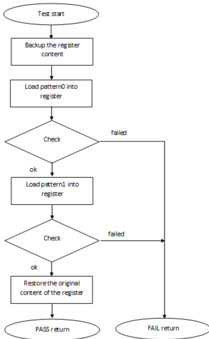
Figure 27. Block diagram for PRIMASK , FAULTMASK, BASEPRI and CONTROL registers test
