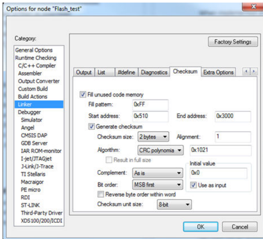
Figure 21. Checksum settings for linker
