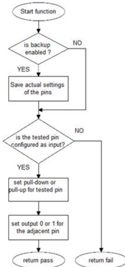
Figure 16. Block diagram of FS_DIO_ShortToAdjSet_IMXRT() function
