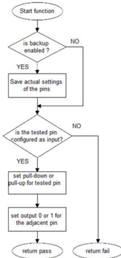
Figure 12. Block diagram of FS_DIO_ShortToAdjSet() function
