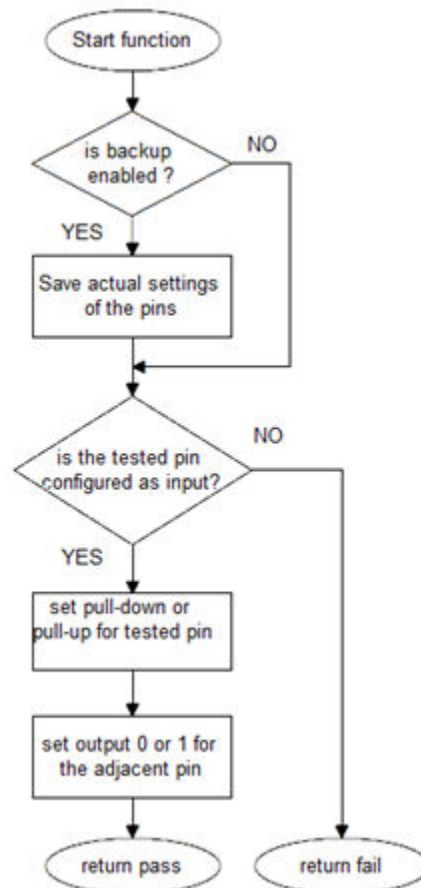
Figure 15. Block diagram of FS_DIO_ShortToAdjSet_LPC() function
