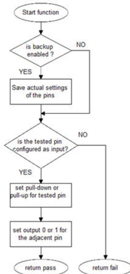
Figure 13. Block diagram of FS_DIO_ShortToAdjSet_IMX8M() function
