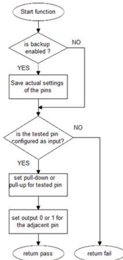
Figure 13. Block diagram of FS_DIO_ShortToAdjSet_IMX8M() function
