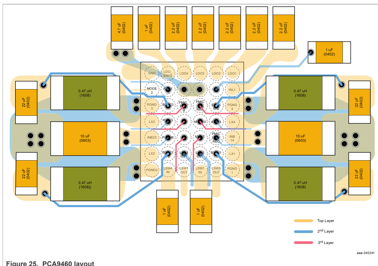
Figure 25. PCA9460 layout
