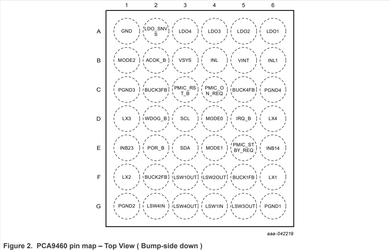
Figure 2. PCA9460 pin map – Top View ( Bump-side down )
