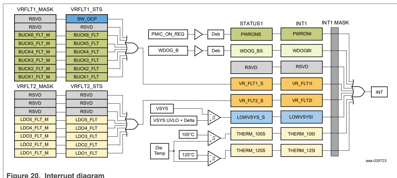
Figure 20. Interrupt diagram
