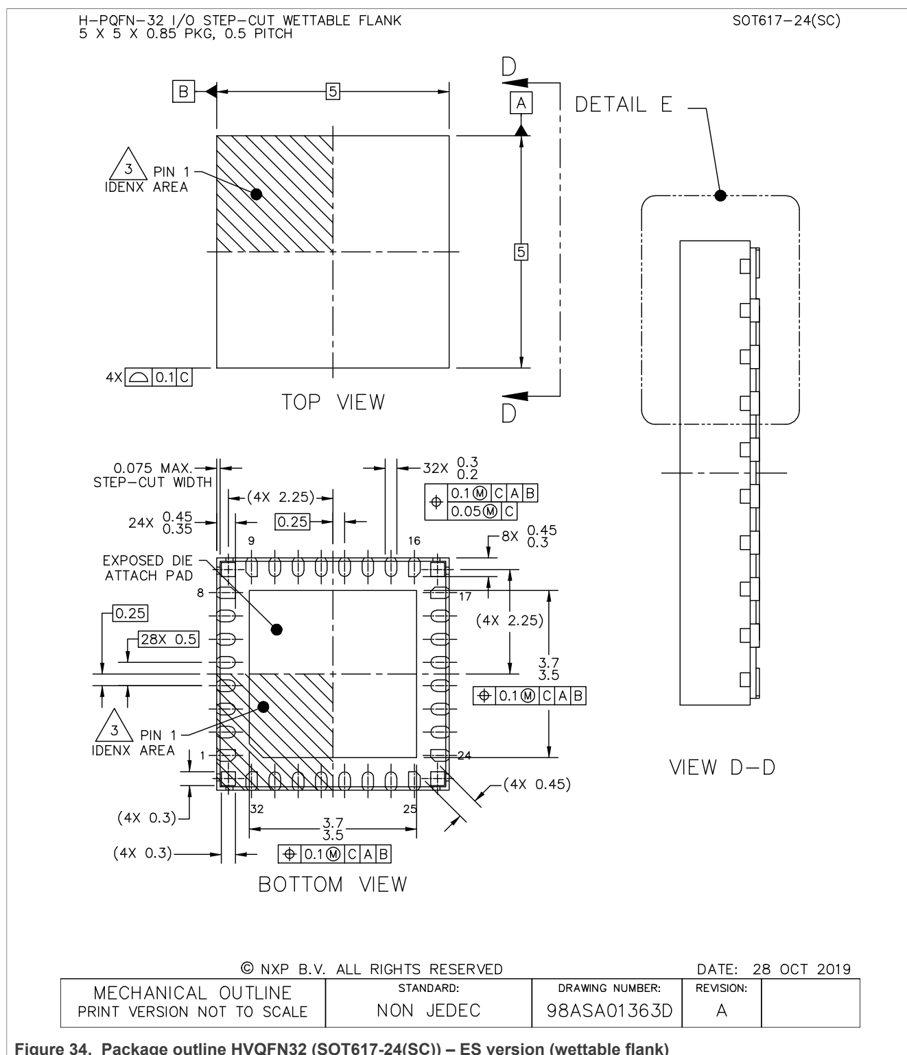
Figure 34. Package outline HVQFN32 (SOT617-24(SC)) – ES version (wettable flank)
