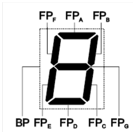
Figure 2. Static LCD
