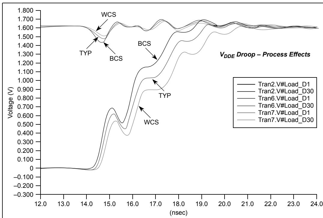
Figure 8. Process
