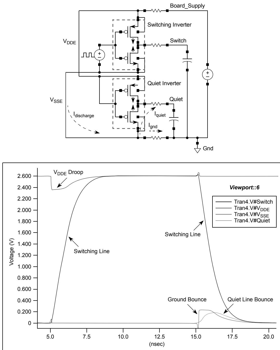
Figure 1. Simple Model with Resistive Return Path
