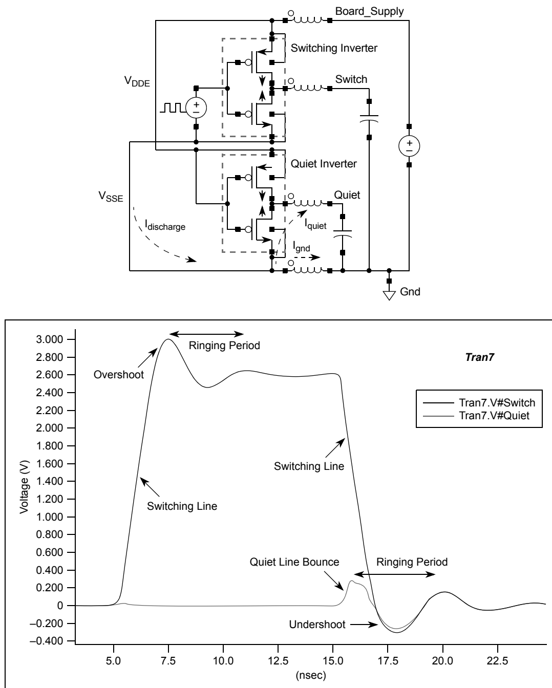
Figure 2. Simple Model with Inductive Return Path
