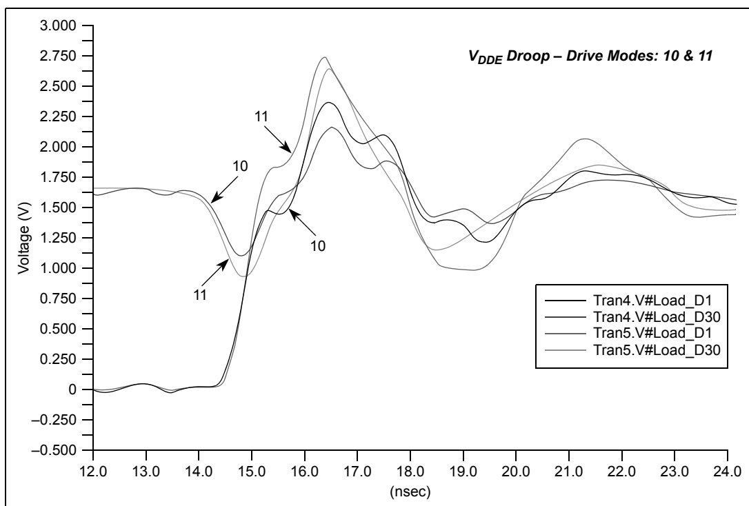
Figure 10. Drive Mode
