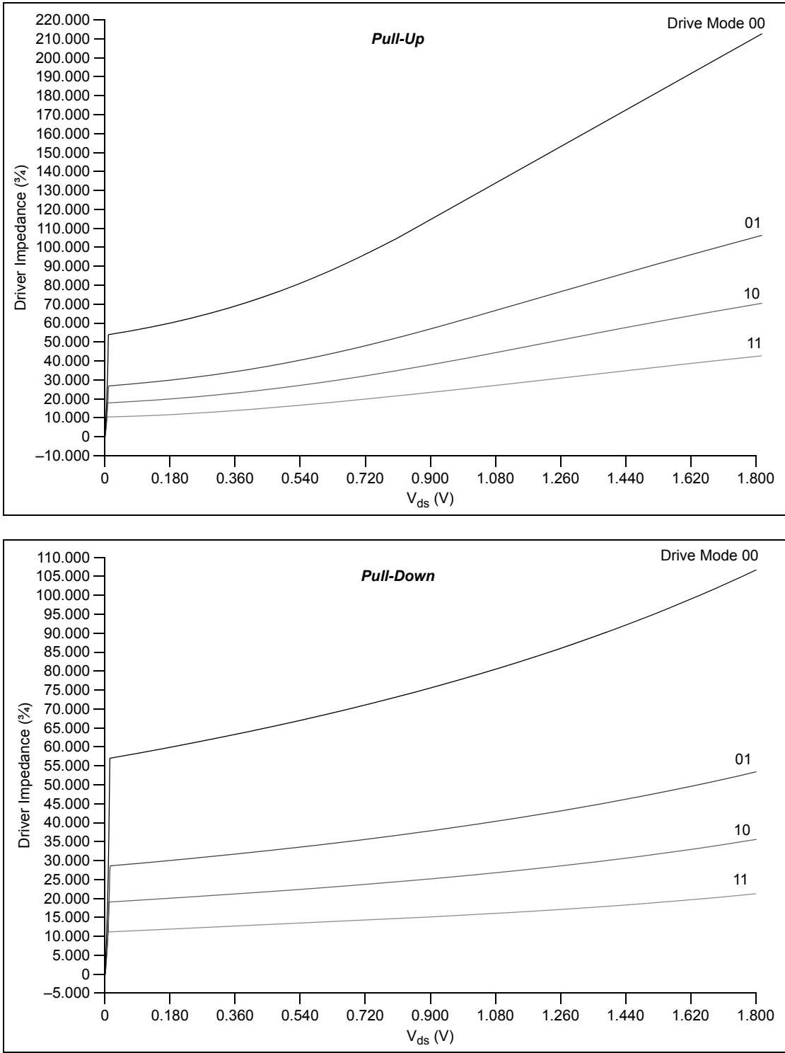
Figure 28. Driver Impedance with VDDE = 1.8V
