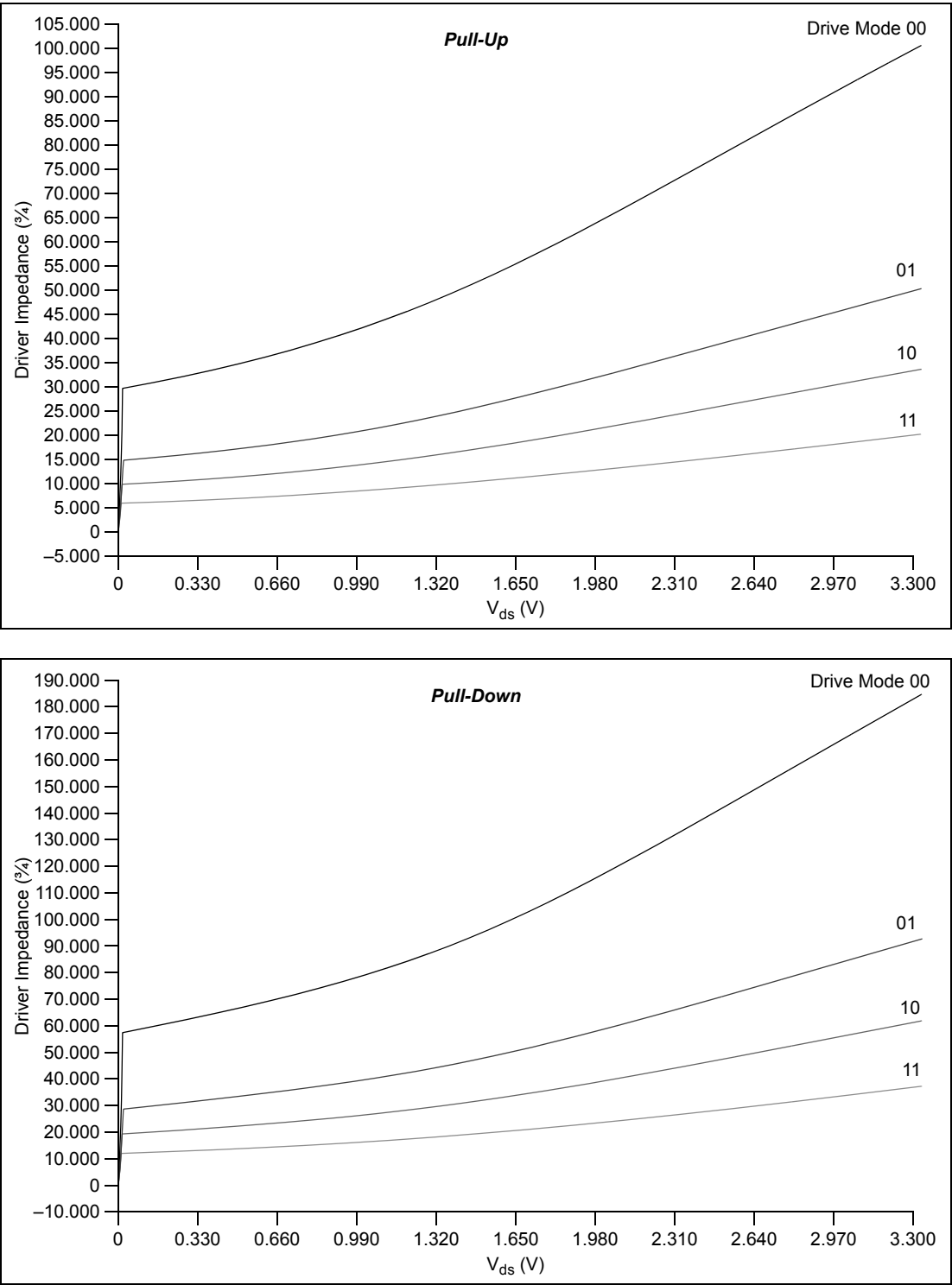
Figure 30. Driver Impedance with VDDE = 3.3V
