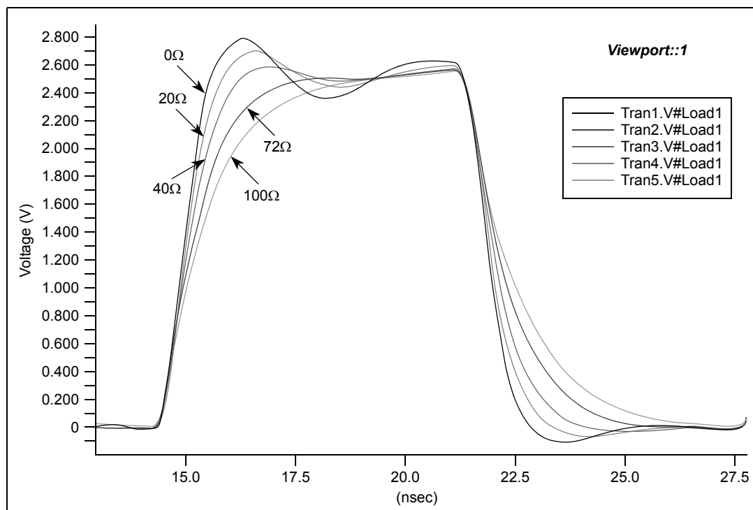
Figure 24. R_T Effect
