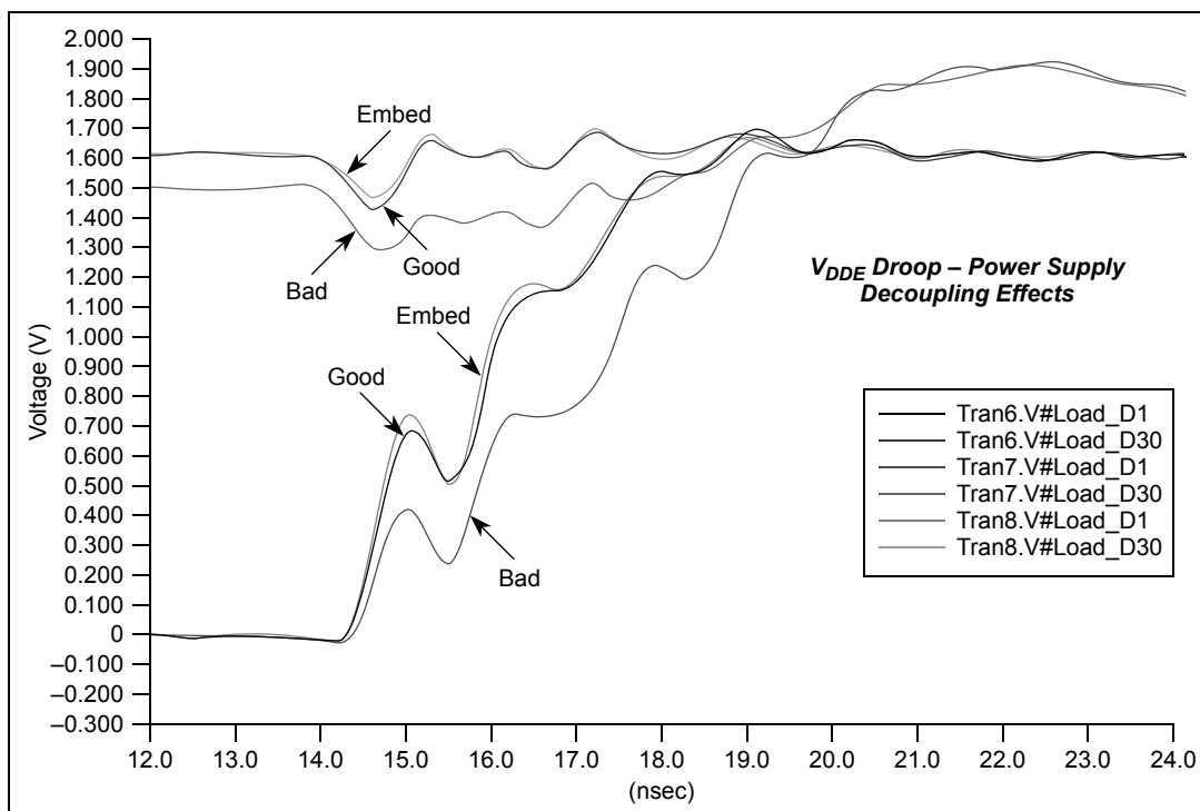
Figure 14. Decoupling Model
