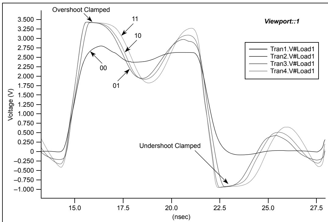
Figure 27. Overdriving Effect
