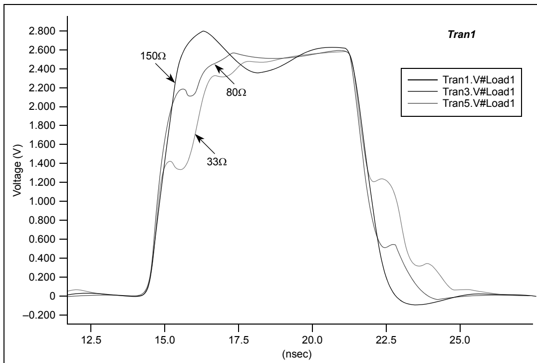
Figure 23. Z_0 Effect
