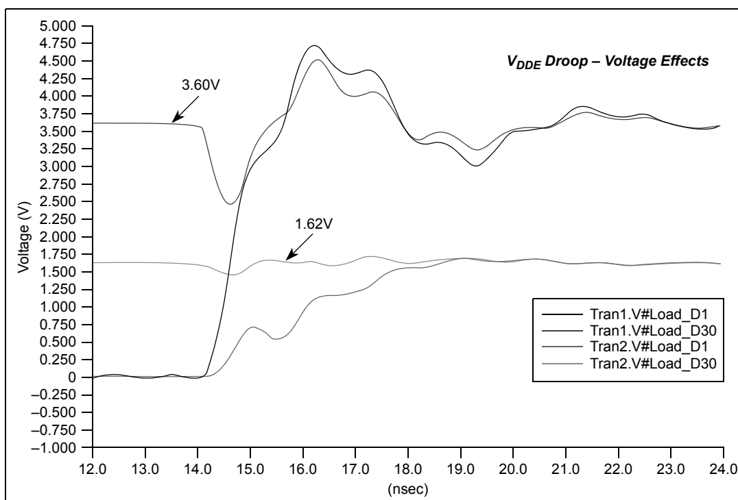
Figure 9. Voltage
