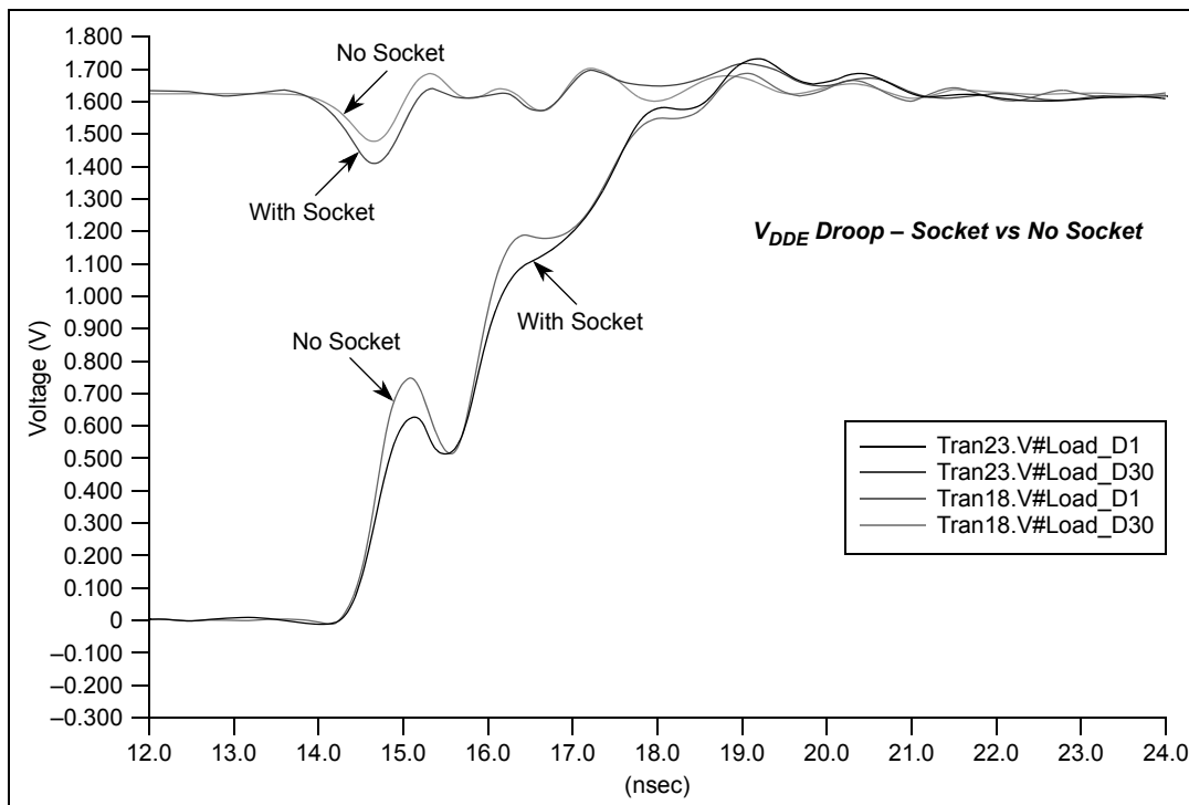
Figure 16. Socket
