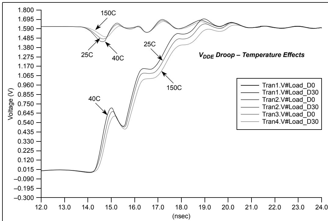
Figure 7. Temperature
