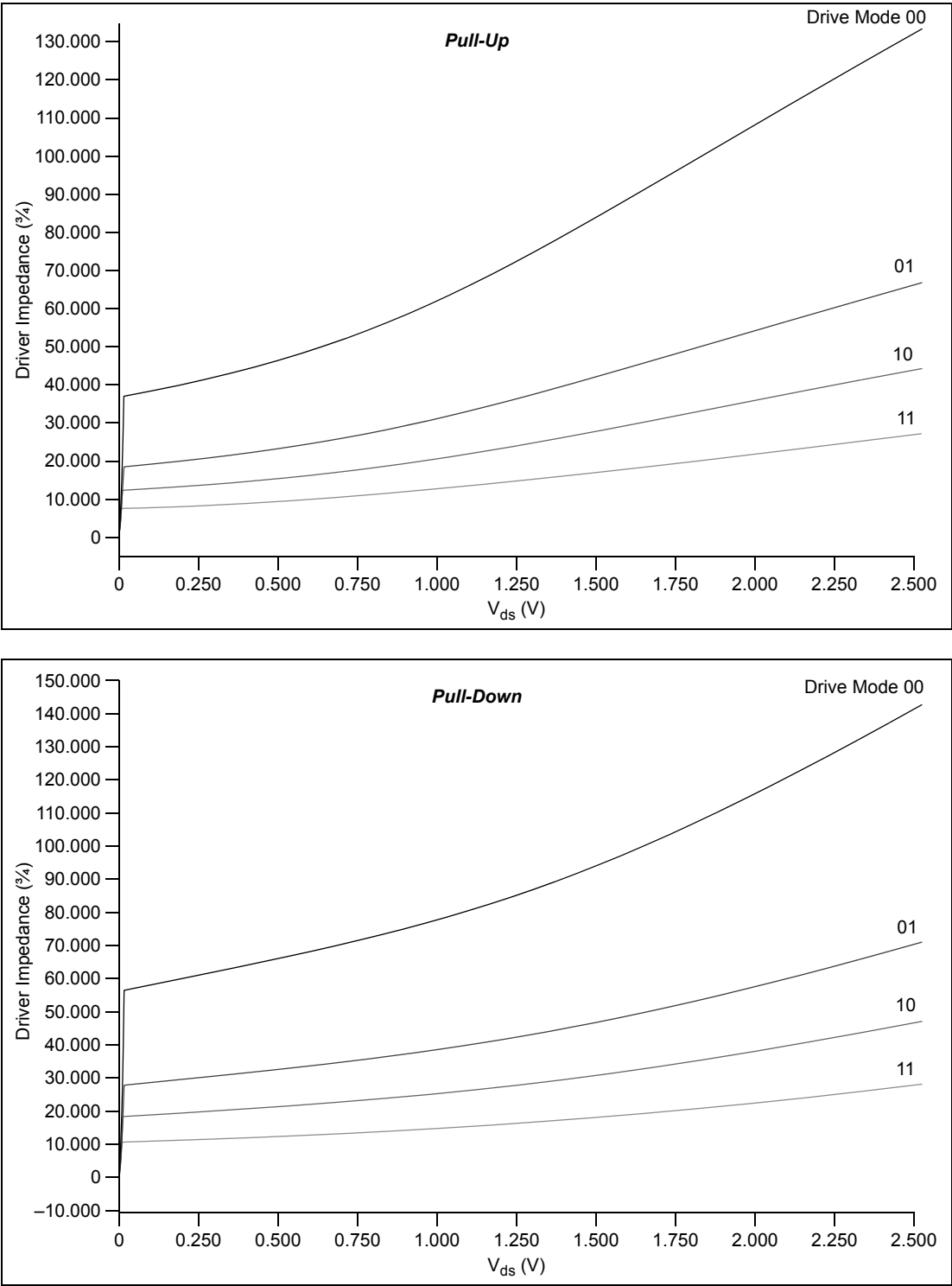
Figure 29. Driver Impedance with VDDE = 2.5V
