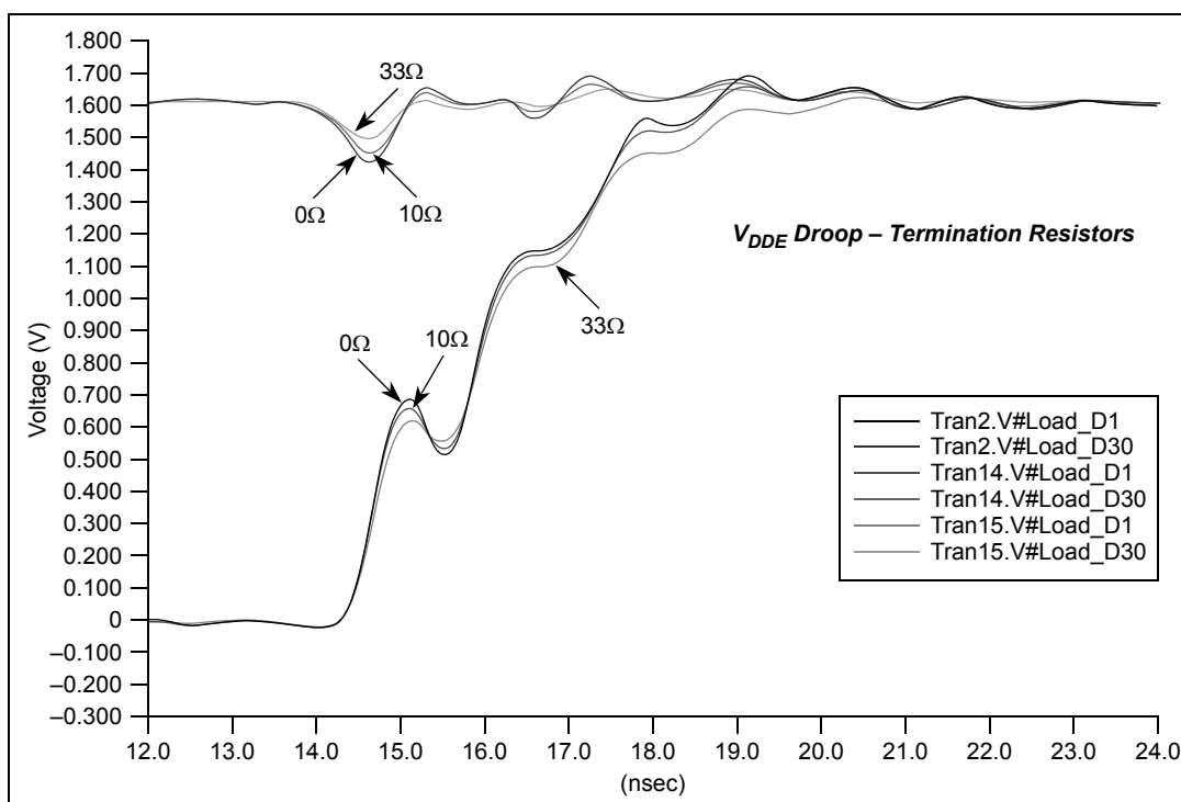
Figure 15. Termination Resistor
