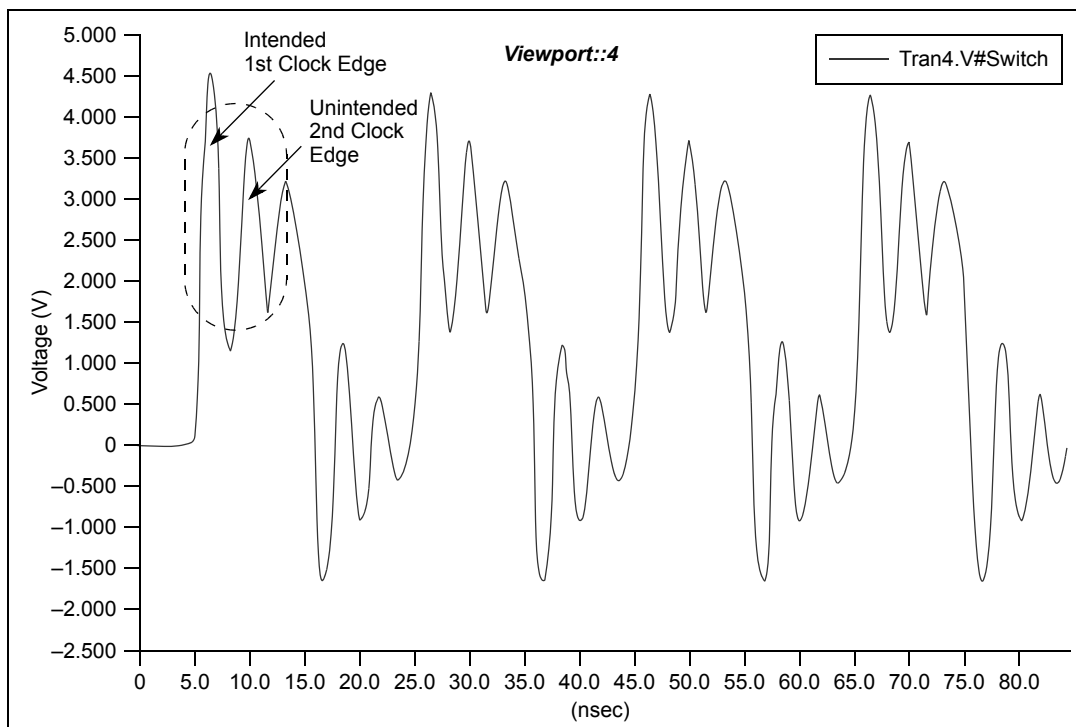
Figure 3. Double Clocking
