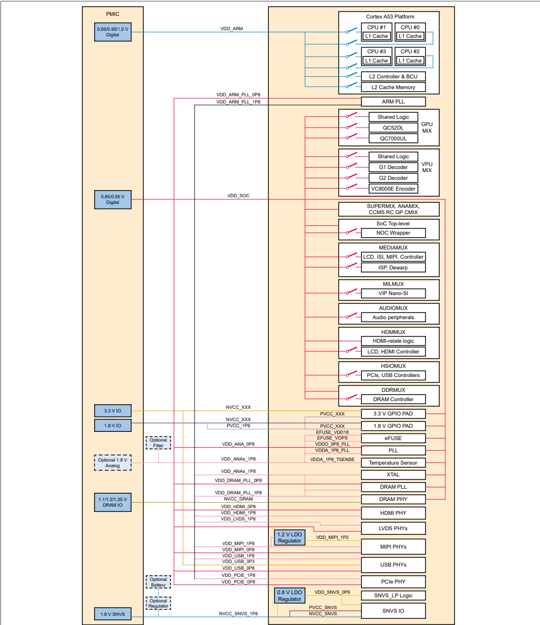
Figure 1. i.MX 8MP power rails
